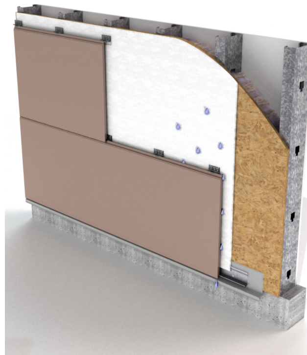
TYPICAL HORIZONTAL PANEL DETAIL
